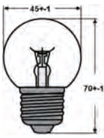
Globe shape G45 Socket E27 Dimensions: 45 *70 mm Tolerance +-1mm
