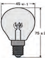
Globe shape G45 Socket E14 Dimensions: 45 *75 mm Tolerance +-1-2mm
